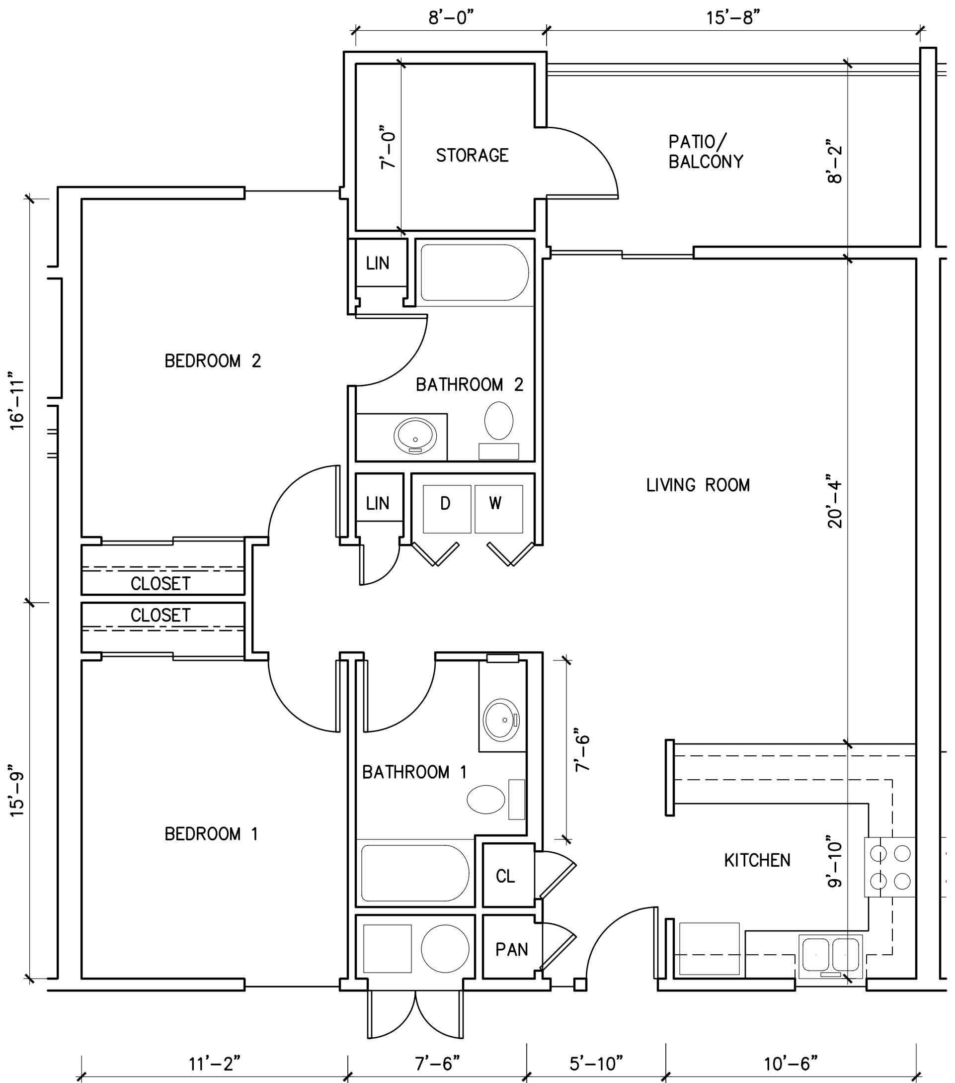
TWO BEDROOM UNIT
